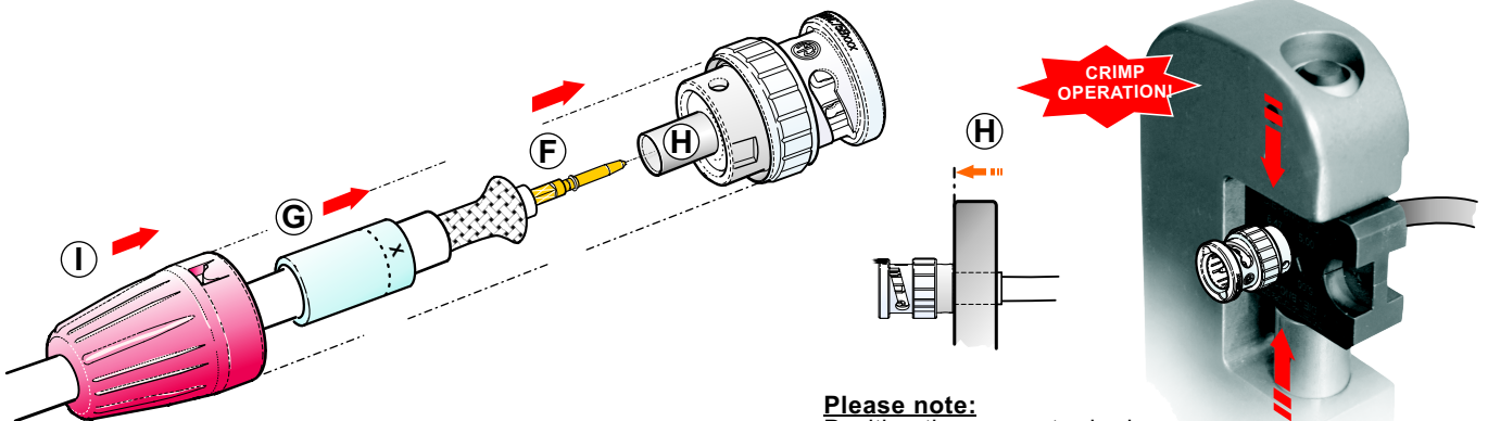
Assembled Connector
