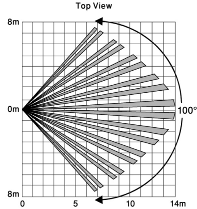
Figure 2: Lens Coverage
